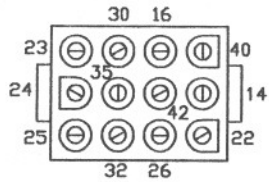
12-TERMINAL MALE PLUG
