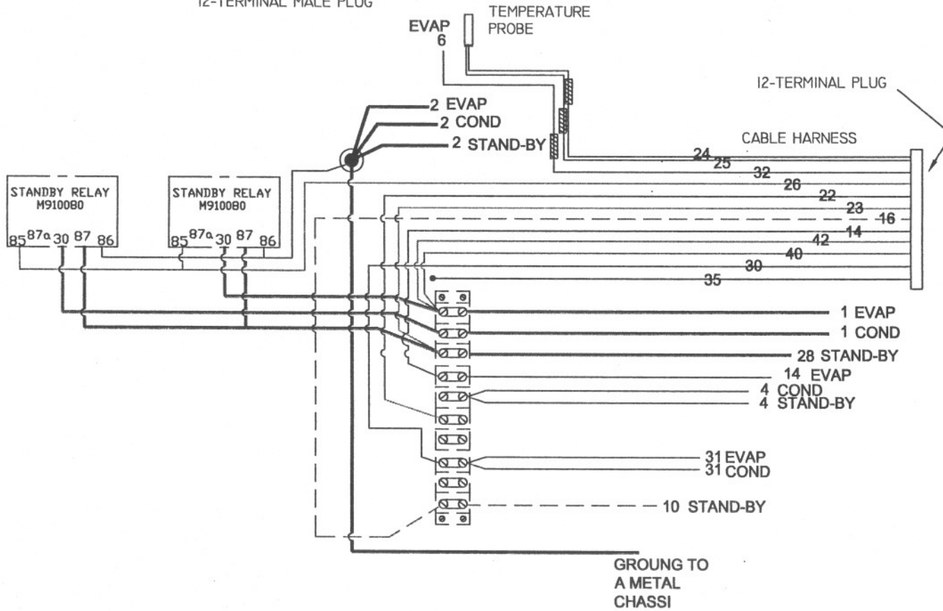
12-TERMINAL MALE PLUG
